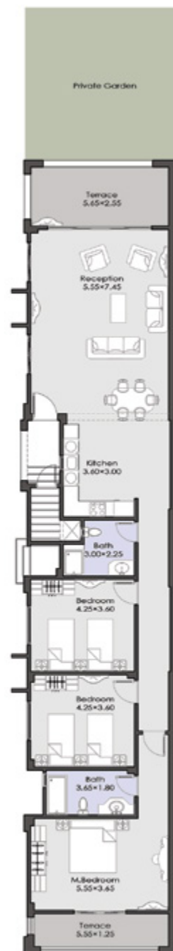
Ground Floor Plan
